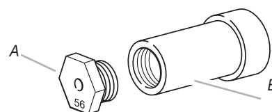
A. LP oven orifice spud stamped with "56" B. Oven Burner Air Shutter
