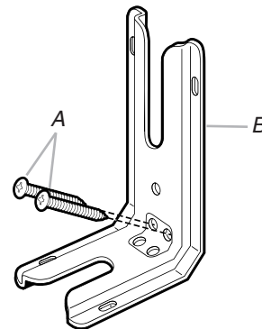
A. #12 x 1\frac{1}{2} " screws B. Anti-tip bracket
