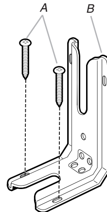
A. #12 x 1\frac{1}{2} " screws B. Anti-tip bracket
