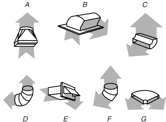
A. Rectangular to round transition piece: 3 1/4" x 10" to 6" = 5 ft (8.3 x 25.4 cm to 15.2 cm = 1.5 m)
