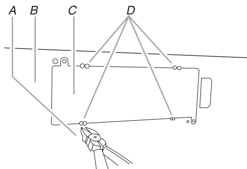
A. Diagonal wire cutting pliers B. Back of microwave oven C. Wall damper vent cover D. Perforations
