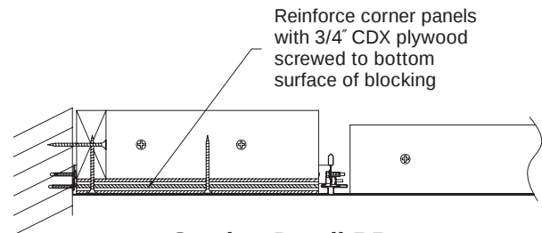
Section Detail BB
