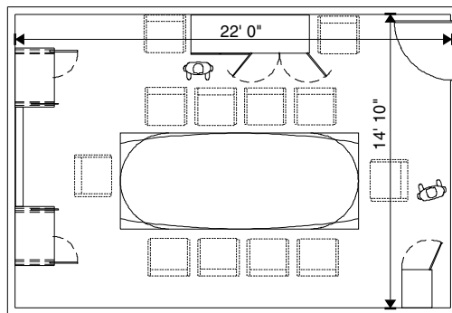
58" x 144" (12') Conference table Seating for 10 to 12 Minimum Room: 20'0" x 12'10" Preferred Room: 21'4" x 14'2"
