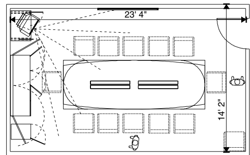
58" x 168" (14') ACT table Seating for 10 to 12 Minimum Room: 22'0" x 12'10" Preferred Room: 23'4" x 14'2"
