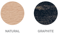
NATURAL GRAPHITE
