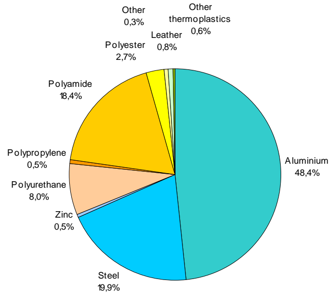
HeadLine with aluminium base, cover Skin, leather armrests (41190322) Cover fabrics will be separated into synthetic materials and natural fibres, depending on the material.
