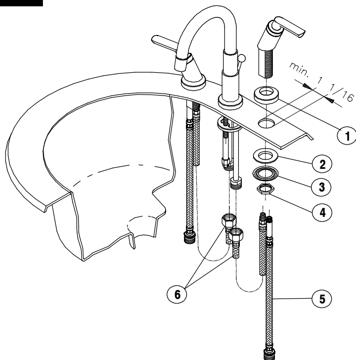
Fig. 2 INSTALLATION OF VALVE ASSEMBLY
