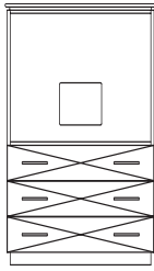
ARMOIRE WITHOUT DOORS EL2436ARO D24 W36 H62
