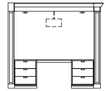
SUITE DIVIDER (RECESSED) 8' CT4399CD D43.5 W99.25 H89.25 10' CT43123CD 11' CT43135CD
