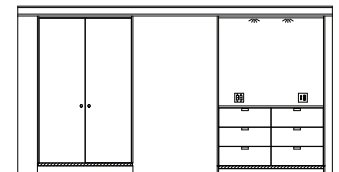
WALL UNIT DRESSER AND WARDROBE 14' CT28168WU3 D24 W168 H89.25
