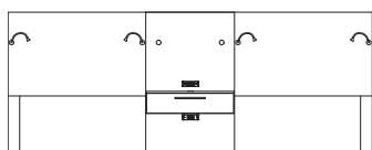
WOOD HEADBOARD DOUBLE HN60156DH-A-02 D18.25 W156 H60 QUEEN HN60170QH-A-02 D18.25 W170 H60
