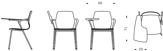
Mezzo Schreibtislar. Mezzo. Writing board.
