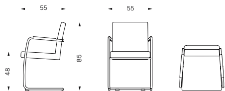
Dexter. Freischwinger. Dexter. Cantilever Chair.
