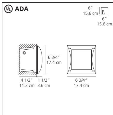
Planar 7" recessed wall
