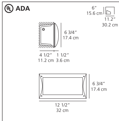
Planar 7" x 13" recessed wall
