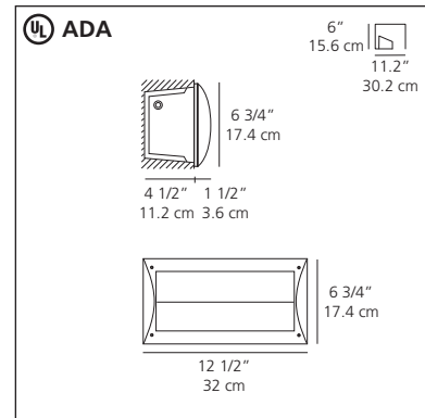
Planar 7" x 13" recessed wall anti-glare shield
