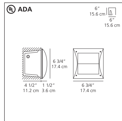
Planar 7" recessed wall anti-glare shield
