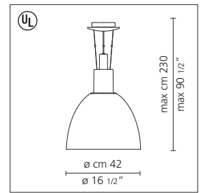
Stranur suspension
