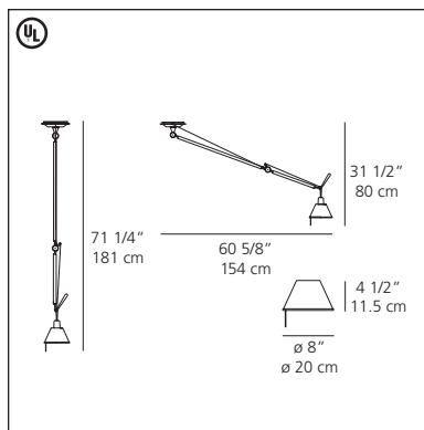
Tolomeo off-center suspension (aluminum diffuser)
