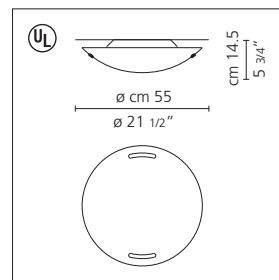
Zsu-Zsu 55 wall/ceiling
