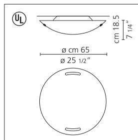
Zsu-Zsu 65 wall/ceiling
