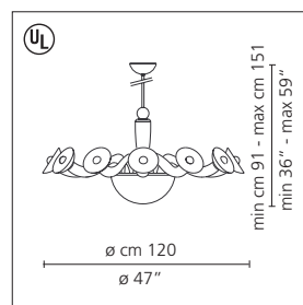
Leda 12 suspension
