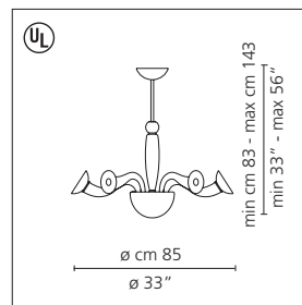
Leda 6 suspension
