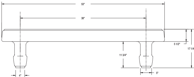
ELEVATION VIEW
