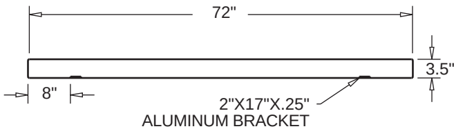
TYPICAL SIDE VIEW
