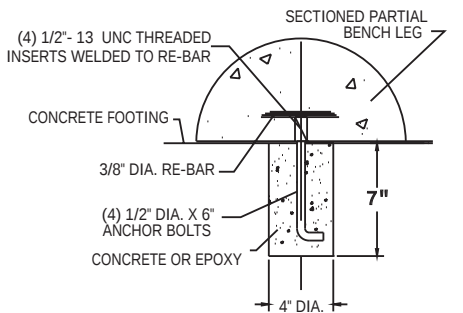
SECTIONED ANCHORING SYSTEM DETAIL
