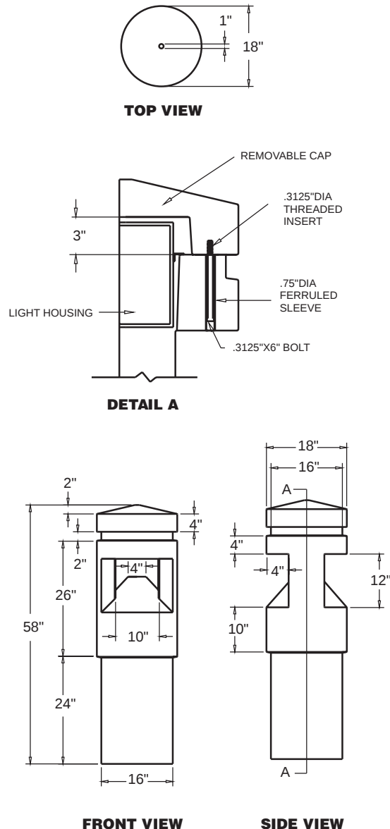
FRONT VIEW
