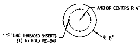
BOTTOM VIEW BOLLARD
