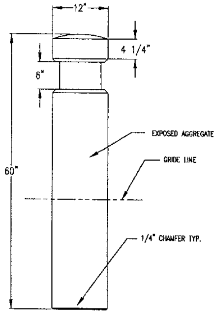
ELEVATION VIEW
