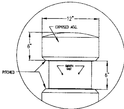
DETAIL BOLLARD BAND
