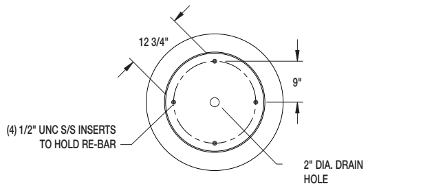
BOTTOM VIEW PLANTER
