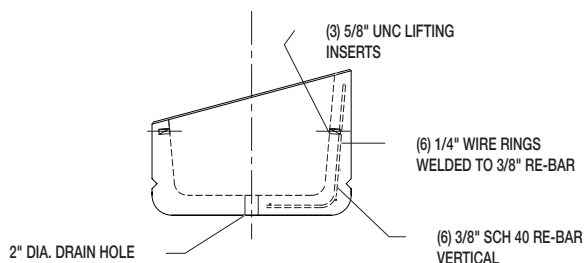
SIDE ELEVATION PLANTER
