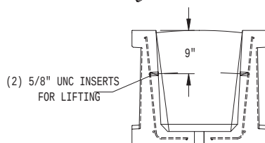
SECTION VIEW
