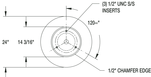
BOTTOM VIEW PLANTER
