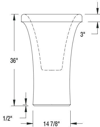
ELEVATION VIEW PLANTER
