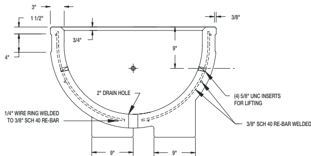
ELEVATION VIEW
