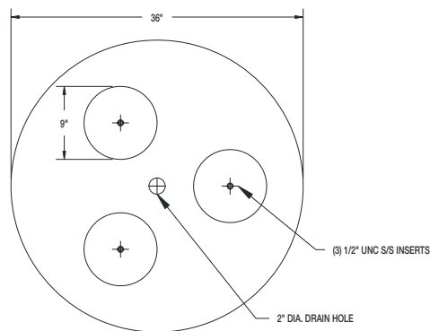
SECTION VIEW PLANTER
