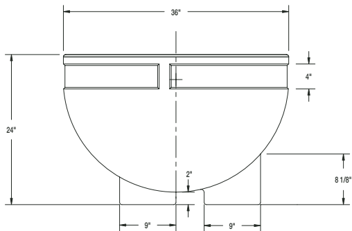
ELEVATION VIEW
