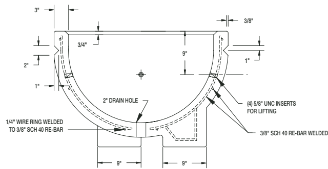
SECTION VIEW PLANTER
