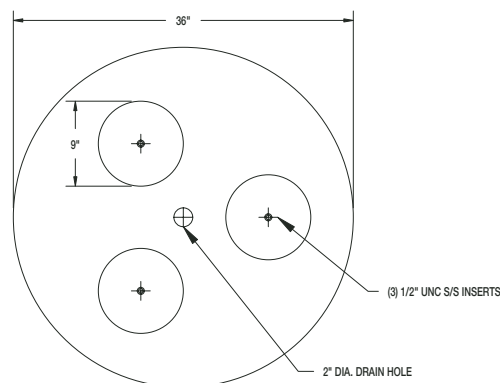
BOTTOM VIEW PLANTER
