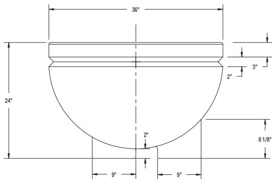
ELEVATION VIEW 90 DEGREES
