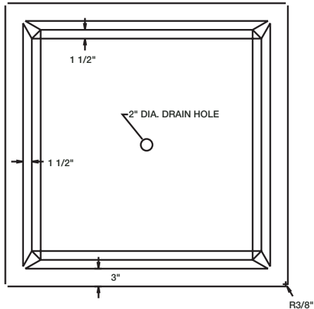
TOP VIEW PLANTER
