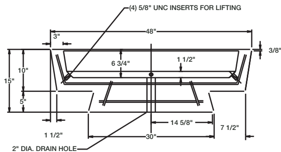
SECTION VIEW PLANTER
