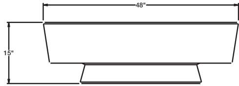
ELEVATION VIEW PLANTER
