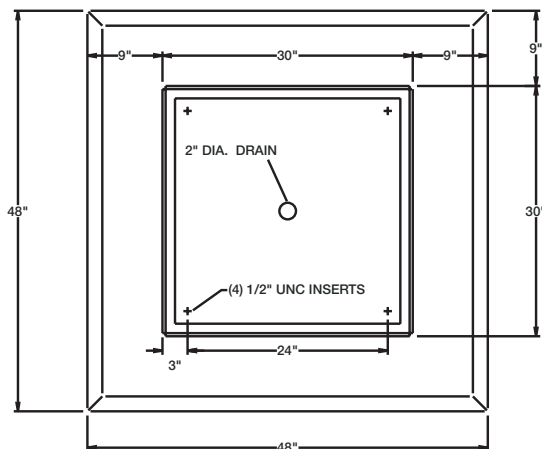
BOTTOM VIEW PLANTER
