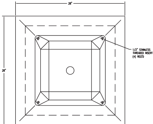
TOP VIEW SCALE: 1/4" = 1"
