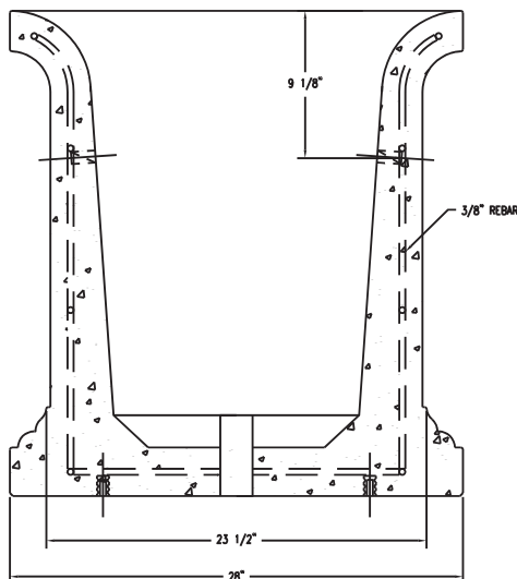
SECTION VIEW SCALE: 1/4" = 1"
