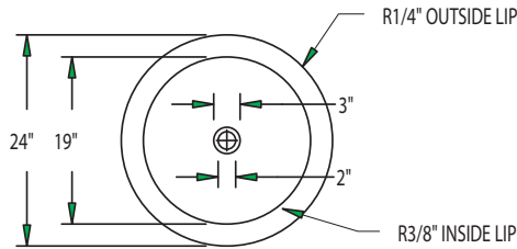
TOP VIEW PLANTER
