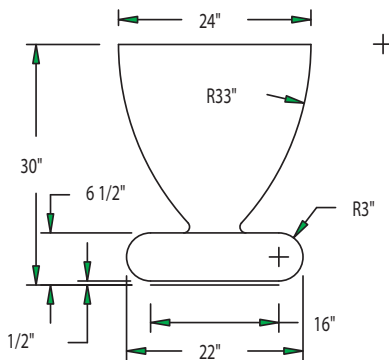
ELEVATION VIEW PLANTER
