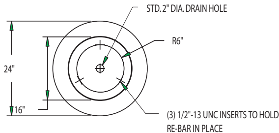
BOTTOM VIEW PLANTER
