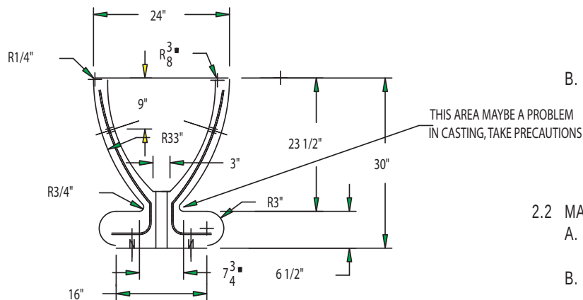
SECTION VIEW PLANTER
