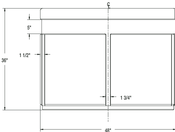
ELEVATION VIEW PLANTER
