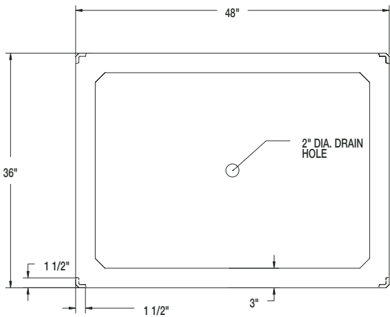
TOP VIEW PLANTER
