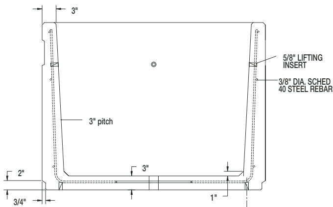
SECTION VIEW PLANTER
