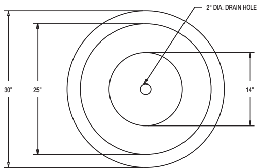
TOP VIEW PLANTER
