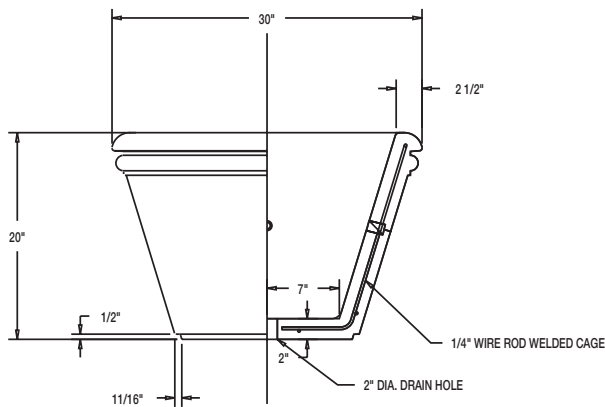
ELEVATION/SECTION VIEW PLANTER
