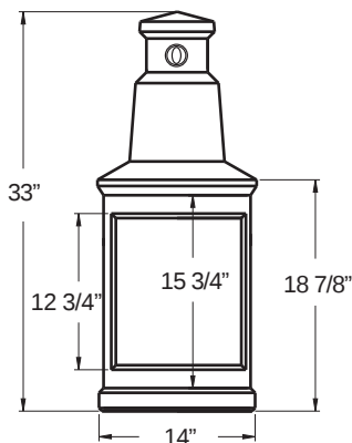
FRONT VIEW SNUFFER
