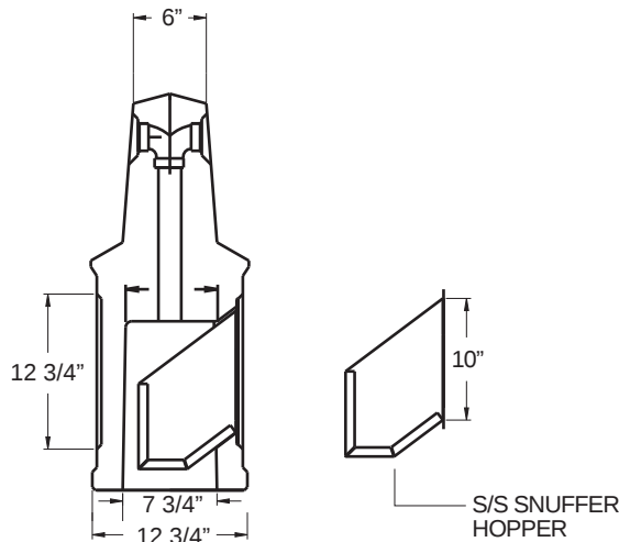
SECTION SNUFFER
