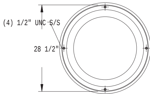
BOTTOM VIEW WASTE CONTAINER
