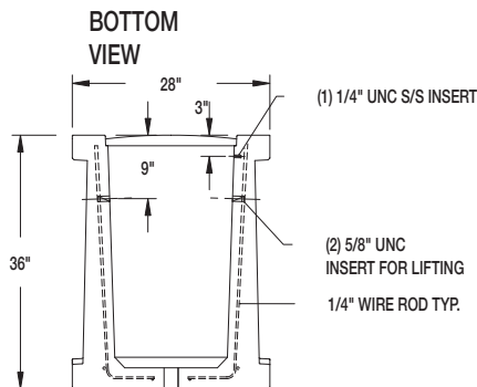
SECTION VIEW
