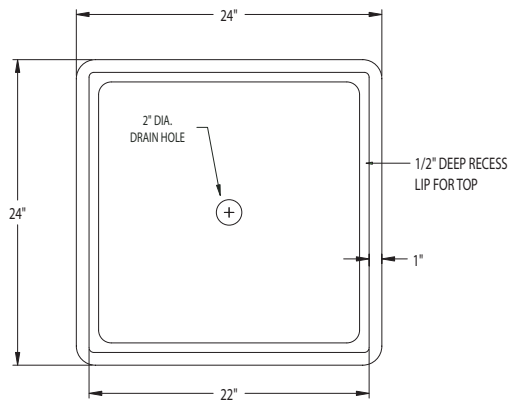
TOP VIEW WASTE CONTAINER
