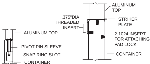
SECTION C-C NOT TO SCALE
