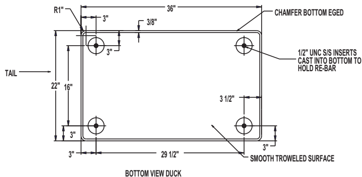
BOTTOM VIEW DUCK
