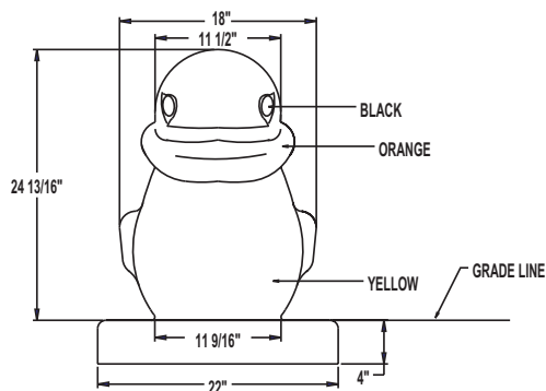
FRONT VIEW DUCK
