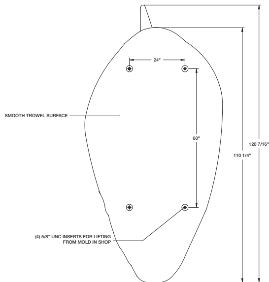
BOTTOM VIEW LOON
