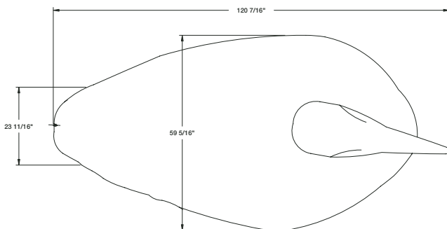
TOP VIEW LOON
