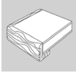
Laminate; 1" x 1-3/4" wood bullnose edge; .62" radius corner (15W)
