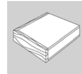
Plus-Laminate; 3/8" x 1-1/4" wood band edge; square corner; corner joint is not mitered (34S)
