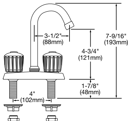
LKA2475 Illustrated
