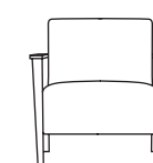
704-1, Chair W-30½", D-31½", H-32½" SH-18", AH-24"
