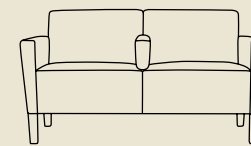
861-25-2, Duet 54 with intervening arm W-54½", D-28½", H-32", SH-18¾", AH-25"
