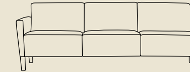
861-30-4, Trio 84 W-84½", D-28½", H-32", SH-18¾", AH-25"
