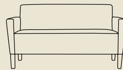
861-2, Duet 54 with continuous cushion W-54½", D-28½", H-32", SH-18¾", AH-25"
