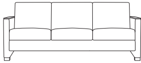
814-30, Three Seat W=82", D=31 1/4", H=26", SH=18", AH=25"
