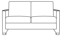
814-20, Two Seat W=57", D=31 1/4", H=26", SH=18", AH=25"
