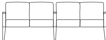
2800-40, Four Seat with full intervening arm W=87", D=26½", H=32½", SH=18¾", AH=25"
