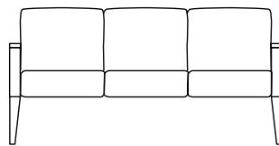
2800-30, Three Seat W=65", D=26½", H=32½", SH=18¾", AH=25"
