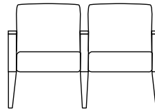
281-22, Two Seat with full intervening arm W=47", D=26½", H=32½", SH=18¾", AH=25"
