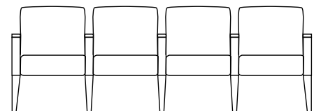
2800-44, Four Seat with full intervening arms W=91", D=26½", H=32½", SH=18¾", AH=25"
