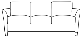
731-30, Three Seat W=77", D=28", H=33 1/4", SH=18", AH=26 1/2"
