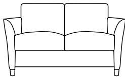
731-20, Two Seat W=55", D=28", H=33 1/4", SH=18", AH=26 1/2"
