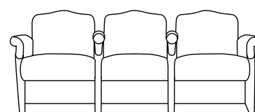
733-33, Three Seat with full intervening arms W=77", D=28¾", H=33" SH=18", AH=24"
