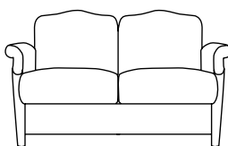
733-20, Two Seat W=52", D=28¾", H=33" SH=18", AH=24"
