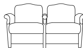
733-22, Two Seat with full intervening arm W=54½", D=28¾", H=33" SH=18", AH=24"
