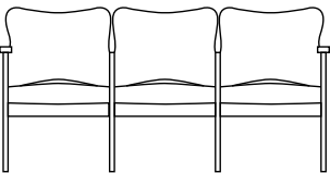
283-30, Three Seat W=66½", D=24½", H=33", SH=18¼", AH=26"
