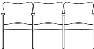
283-33, Three Seat with full intervening arms W=66½", D=24½", H=33", SH=18¼", AH=26"
