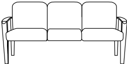
2750-30, Three Seat W=64½", D=25", H=33¾", SH=18¼", AH=25½"
