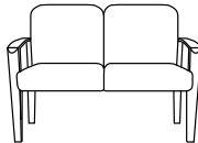
2750-20, Two Seat W=44½", D=25", H=33¾", SH=18¼", AH=25½"
