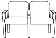
2750-22, Two Seat with full intervening arm W=46", D=25", H=33¾", SH=18¼", AH=25½"
