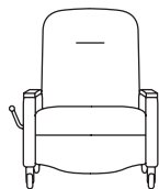
PRCL-130B, Bariatric Recliner W=37", D=38", H=48" SH=21", AH=25" Seat Width=28"
